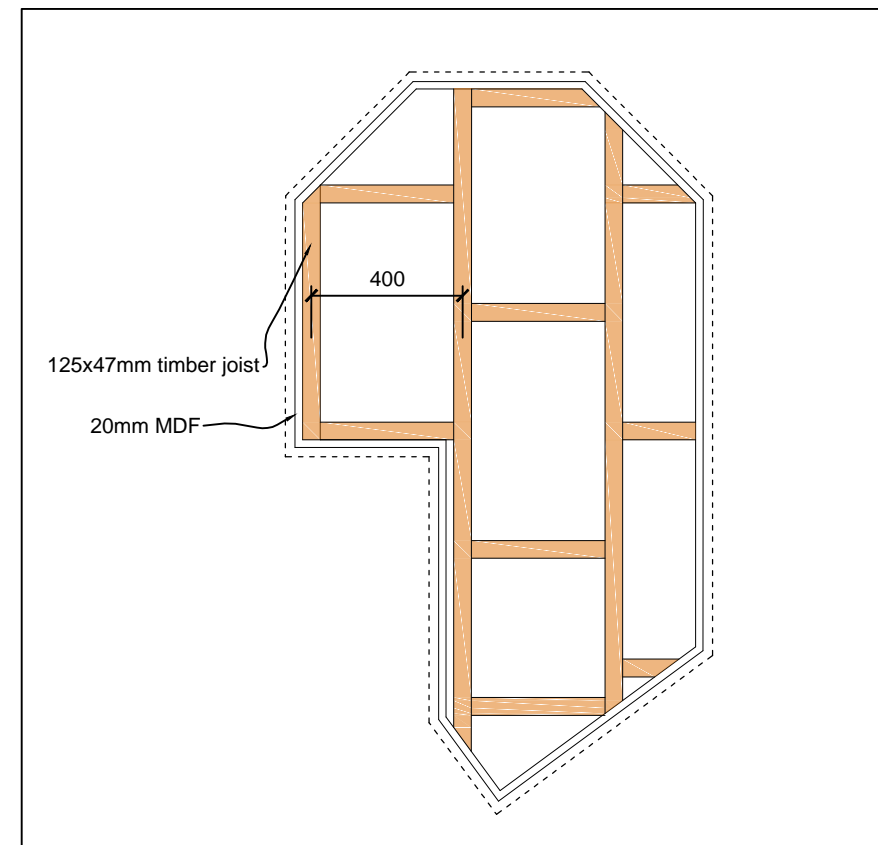
DETAIL PLAN 1:20
