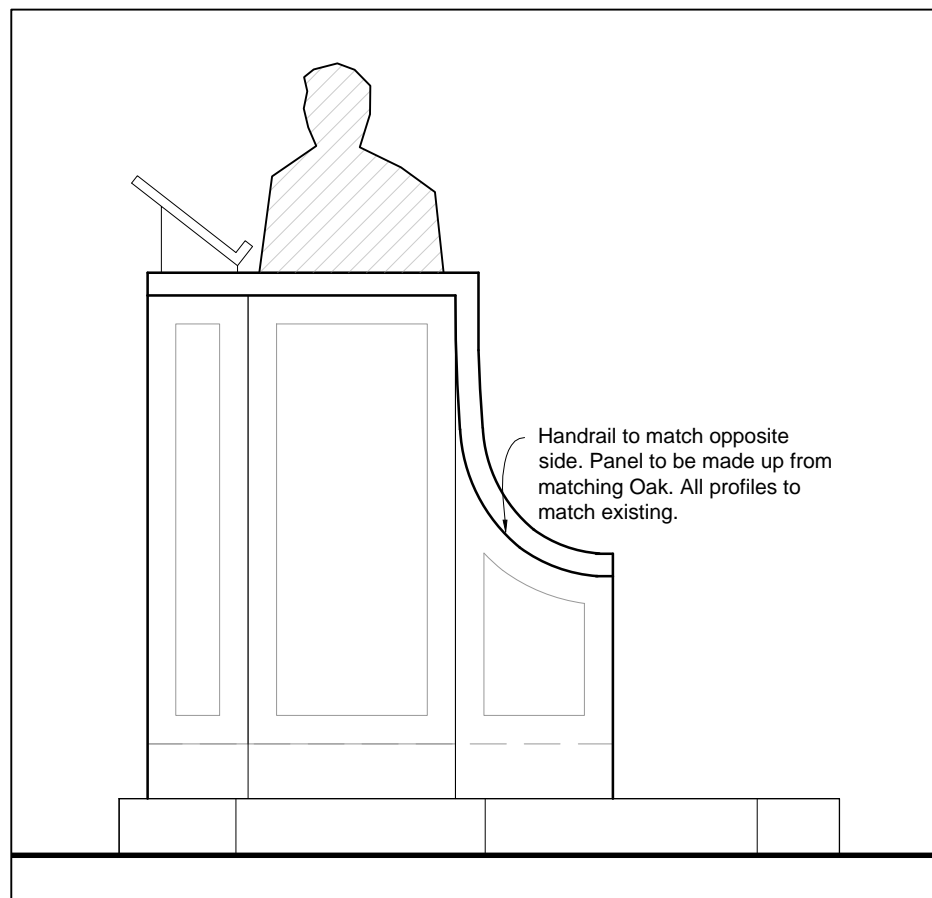
ELEVATION A 1:20
