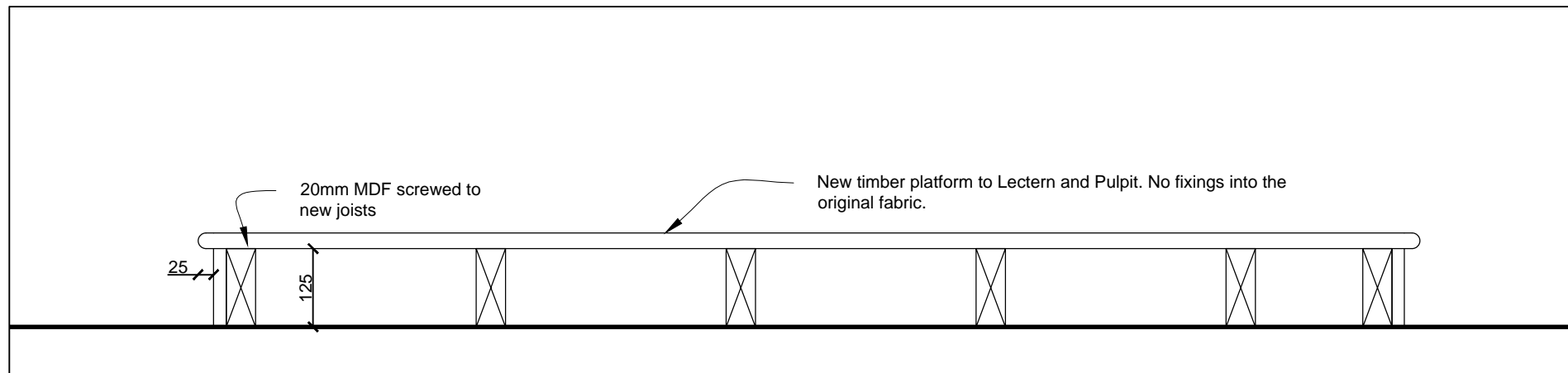
DETAIL SECTION 1:10
